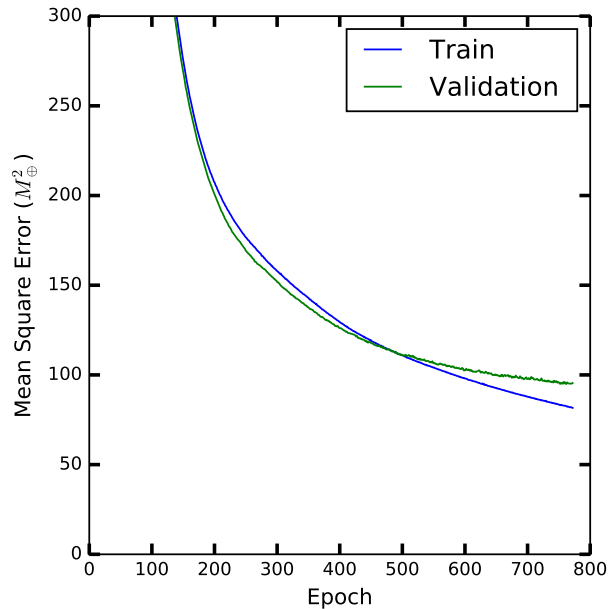
Figure 8. Training and validation loss as a function of training epoch for the DPNNet for computation of the planet mass.
