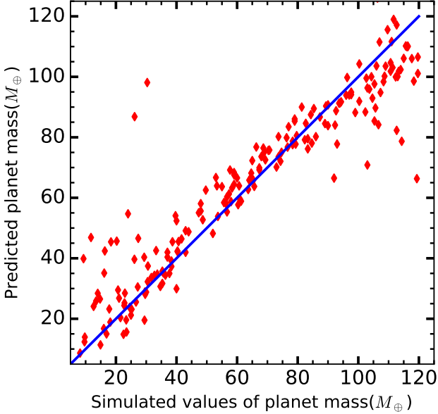
Figure 5. Correlation between the predicted planet mass (in the units of M_{\oplus} ) using DPNNet and the simulated planet mass used in the numerical simulations.
