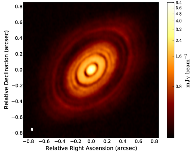
Figure 1. ALMA continuum image of HL Tau (ALMA Partnership et al. 2015). The synthesized beam is shown in the lower left. Adapted from Dipierro et al. (2015).
