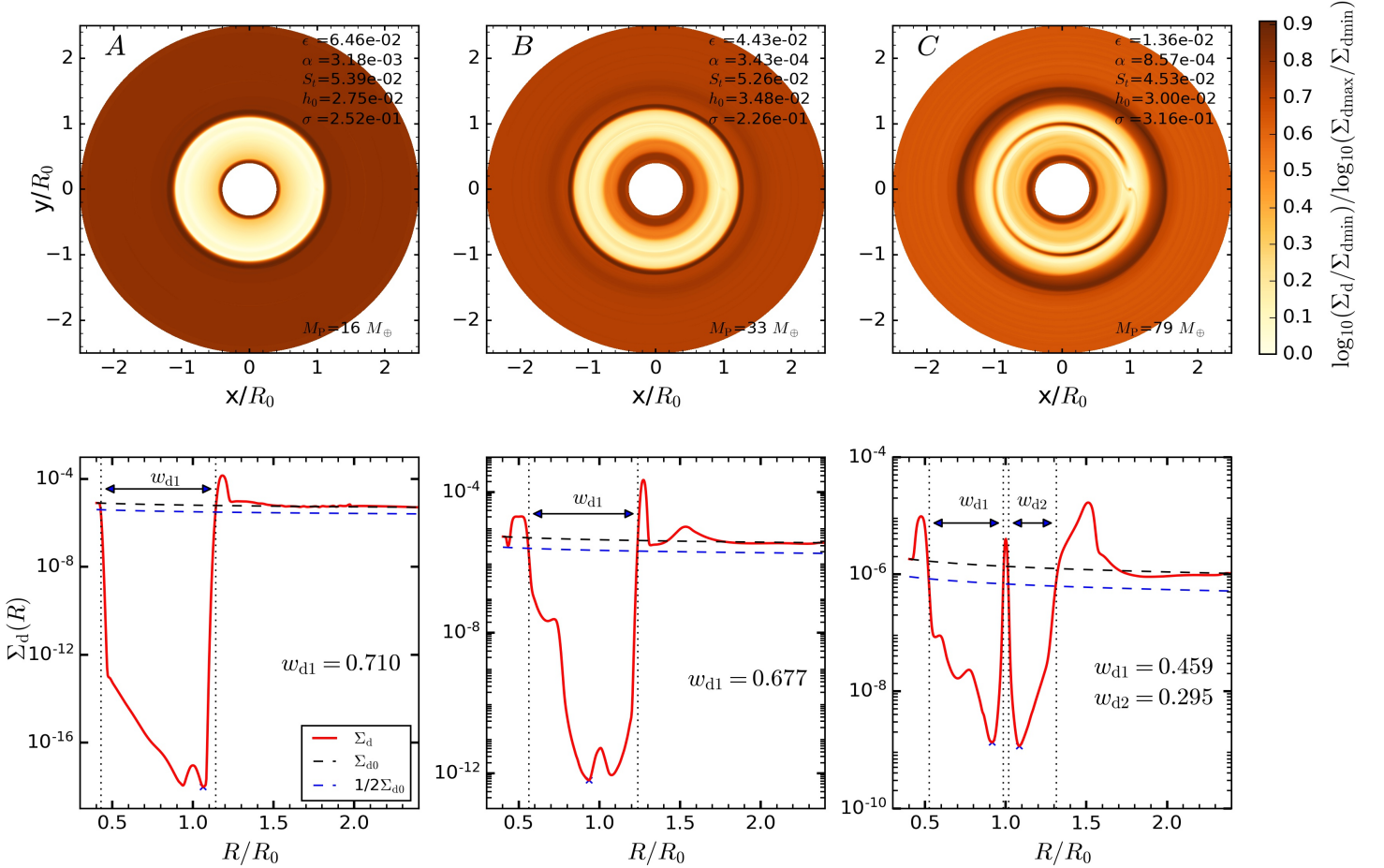
Figure 3. The top panel is the normalized dust surface density distribution after 3 \times 10^3 orbits for different planet masses and different disk initial conditions. The disk parameters for each model are indicated on the top right of each plot. The bottom panel is the radial profile (red line) of the azimuthally averaged surface density for each simulation. The horizontal arrow represents the widths w_{d1} , w_{d2} of the gap(s). The gap width is the distance between the inner and the outer edge of the gap (vertical dotted lines) where \Sigma_d(R) reaches 50% of the initial surface density \Sigma_{d0} shown in dotted blue line. The cross indicates the minimum surface density \Sigma_{dmin} .
