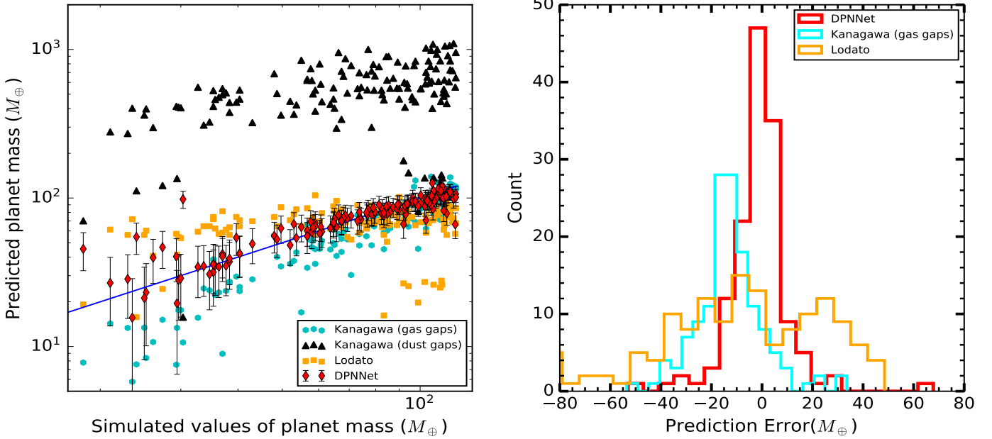
Figure 7. Comparison between the planet mass predicted using different models and the simulated planet mass. The DPNNet-predicted mass lies along the blue line indicating close correlation with the true mass. The black triangles are the predicted mass using Kanagawa model from dust gap width, i.e., setting w_g \rightarrow w_{d1} in Eq. 2. The Kanagawa models overestimate the planet mass. The orange squares are the inferred mass from Lodato model (Eq. 1). They deviate considerably from the simulated values both in the low and high mass end. The masses inferred (cyan hexagon) from kanagawa model using gas gap widths (Eq. 2 without modification) are marginally below the blue line near the low mass end, indicating under prediction. Right: Distribution of the prediction error ( M_{P,simulation} - M_{P,predicted} ) for Kanagawa, Lodato and DPNNet with ( \mu = -12.7M_{\oplus} , \sigma_E = 13.1M_{\oplus} ), ( \mu = -7.4M_{\oplus} , \sigma_E = 31.2M_{\oplus} ) and ( \mu = -1.2M_{\oplus} , \sigma_E = 12.0M_{\oplus} ) respectively.
