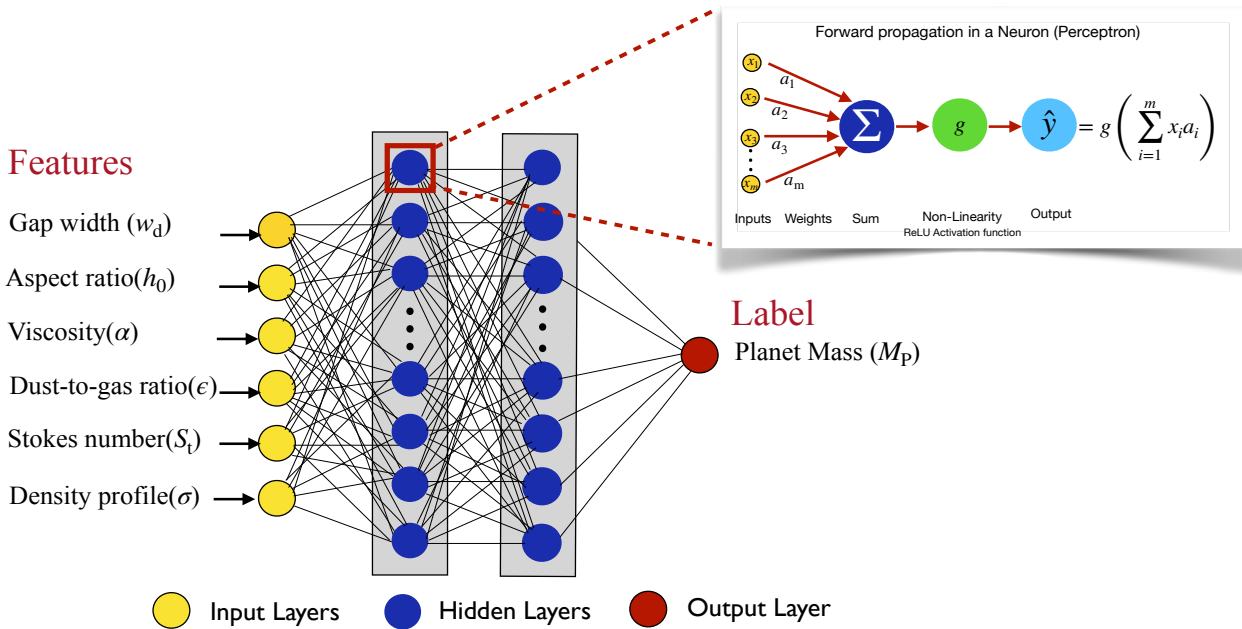
Figure 2. The schematic diagram of the DPNNet using a fully connected multi-layer perceptron. The first layer in yellow takes as input six feature variables. The output layer in red gives the planet mass as a target variable. The two hidden layers in the middle (in blue) has 128 units of neurons each. Each neuron performs a simple task via forward propagation illustrated in the zoomed panel. It finds the linear combination of inputs (weighted sum) and then passes it through a ReLU activation function to generate an output. The network is trained using RMSprop optimizer. More details in §3.
